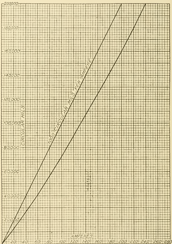
Fig. 1. Curves Showing Safe Carrying Capacity of Copper Wires
